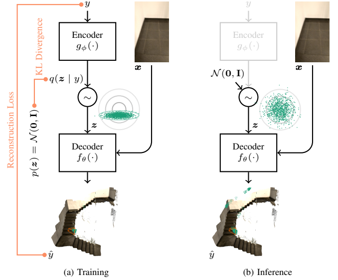
Fig. 2. (a) Our pose generative model is trained as the decoder in a conditional variational autoencoder pipeline reconstructing the ground-truth pose y \in \text{SE}(3) for an image x \in \mathbb{R}^{H \times W \times 3} . The loss terms used in the learning objective are shown in orange. During training the latent posterior only partly overlaps with the latent prior, resulting in generated pose samples concentrated at the ground-truth pose. (b) At inference time latent samples are drawn from the prior distribution and mapped to distinct modes in \text{SE}(3) . In the 3D rendering of the scene we can see that for the query image viewing an ambiguous landing at the staircase, output pose samples are concentrated at three modes looking at different, but visually similar landings, including the ground truth. Pose samples are shown by teal and the ground truth by orange camera frusta.
